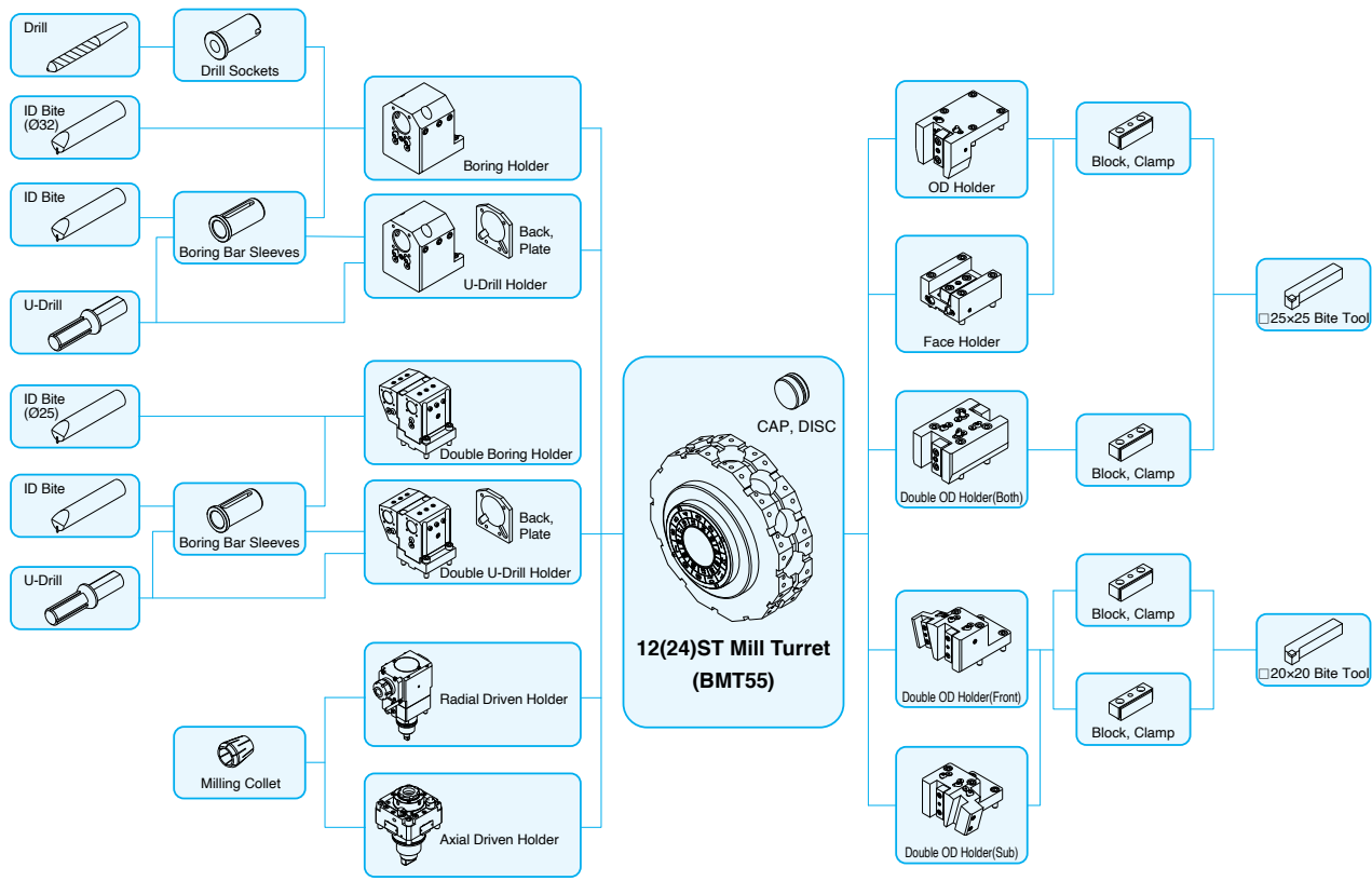
Standard Tooling (NS 2600SY series)
