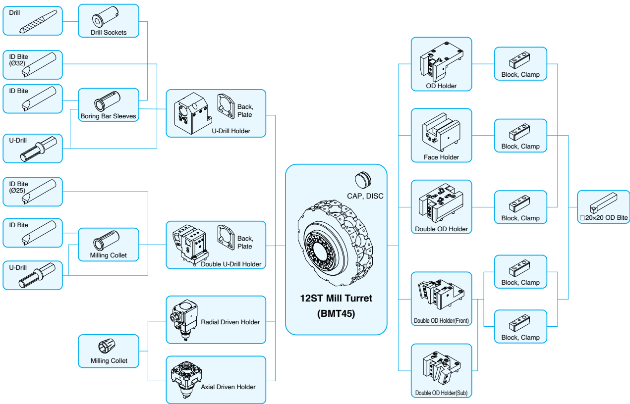
Standard Tooling (NS 2100SY series)
