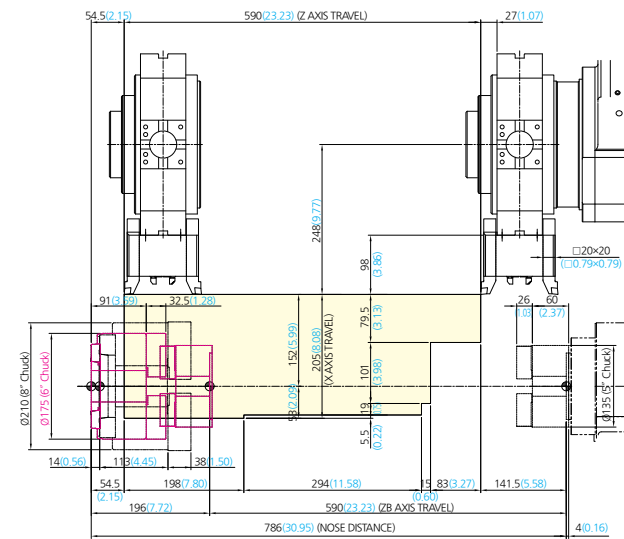
DOUBLE O.D HOLDER_BOTH SIDE (MAIN)
