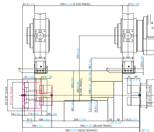
DOUBLE U-DRILL HOLDER (MAIN)
